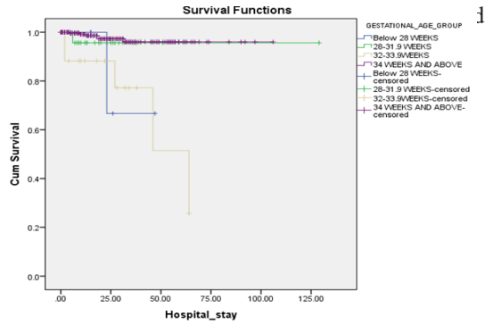
Figure 2: Kaplan Meier curve (gestational age at birth) of surviving preterm newborns (Log Rank (Mantel -Cox): \chi^2 : 27.460 and p < 0.001 )
