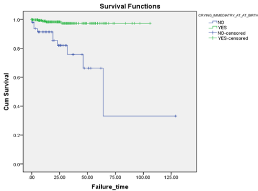
Figure 2: Kaplan Meier curve (by crying immediately after birth) of surviving preterm newborns (Log Rank (Mantel -Cox): \chi^2 : 28.114 and p < 0.001 )
