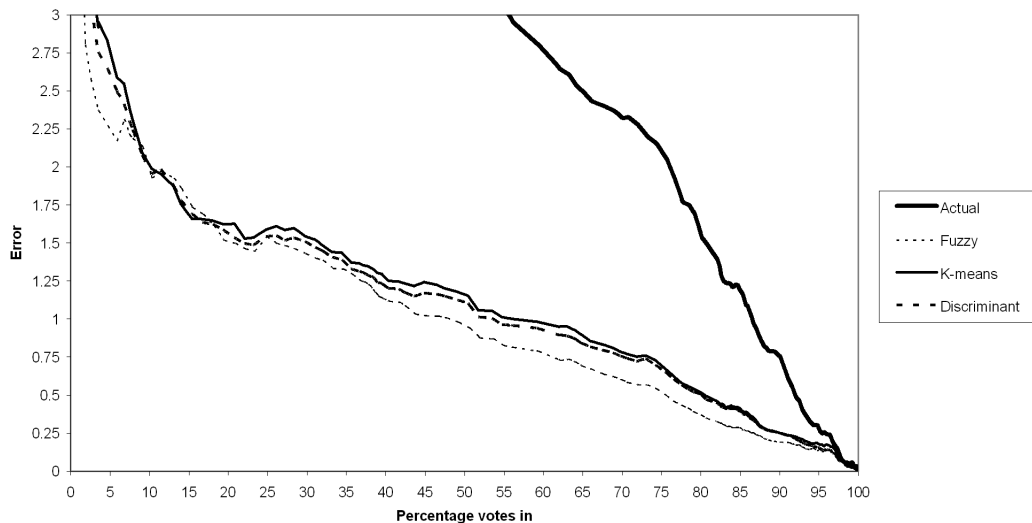
Figure 4: Comparison of the average error E(t) for three cluster methods used in the predictions of the 2004 national election results (based on clusters developed from the 1999 results).
