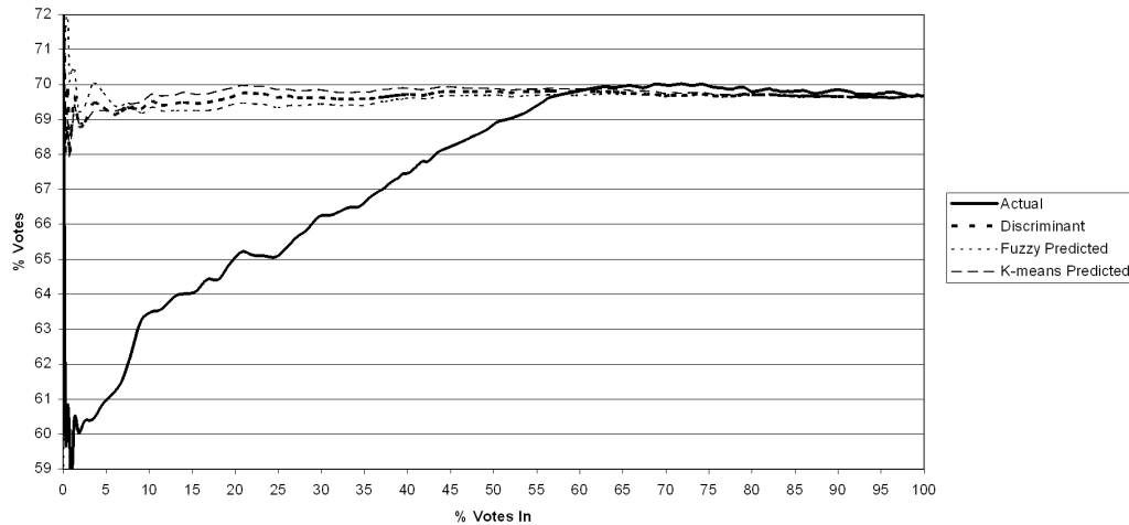
Figure 1: ANC results for the national elections in 2004 and their predictions as a function of the number of votes counted.
