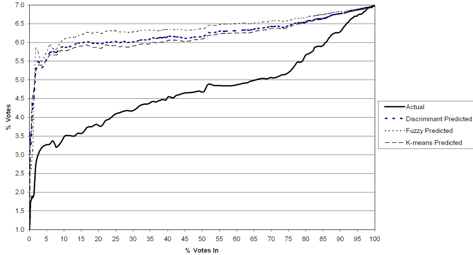
Figure 3: IFP results for the national elections in 2004 and their predictions as a function of the number of votes counted.
