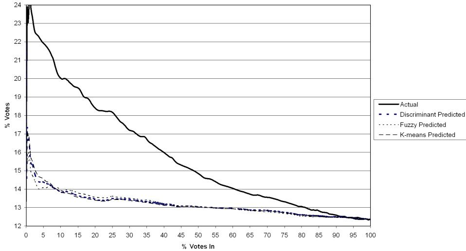
Figure 2: DA results for the national elections in 2004 and their predictions as a function of the number of votes counted.
