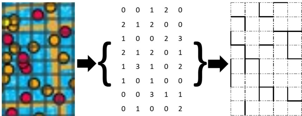
Figure 12: Example of the maze generation process using a matrix
