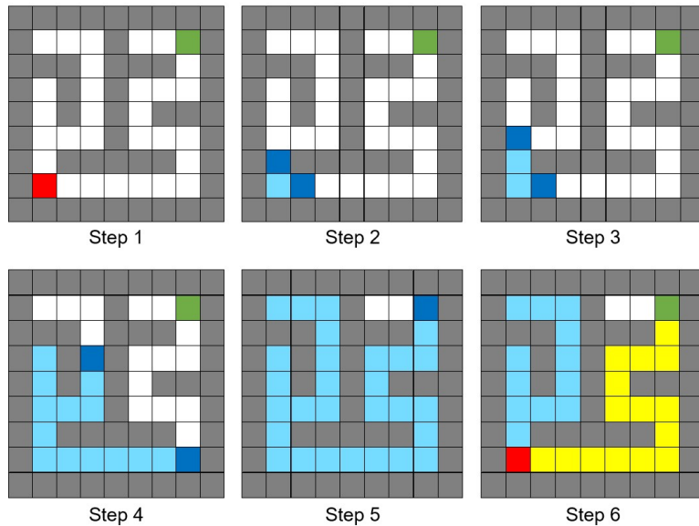
Figure 6: Maze solution generated by the Lee algorithm
