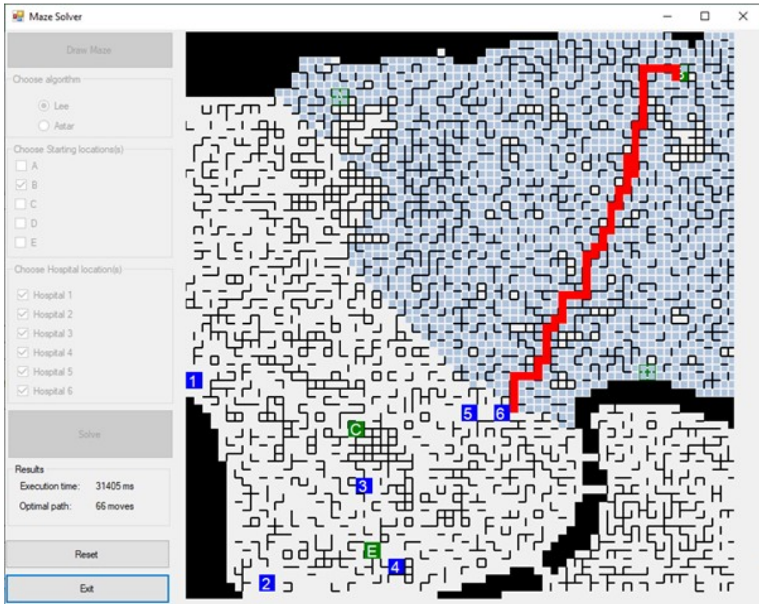
Figure 15: Optimal route generated by the Lee algorithm
