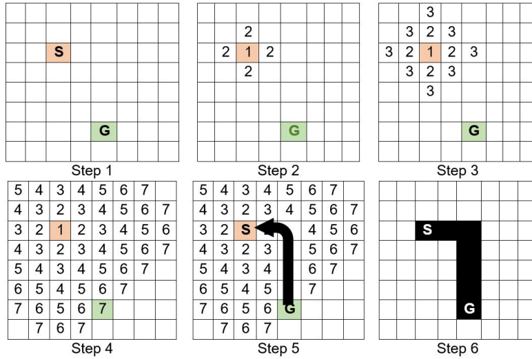
Figure 5: The filling and retrace stages of the Lee algorithm
