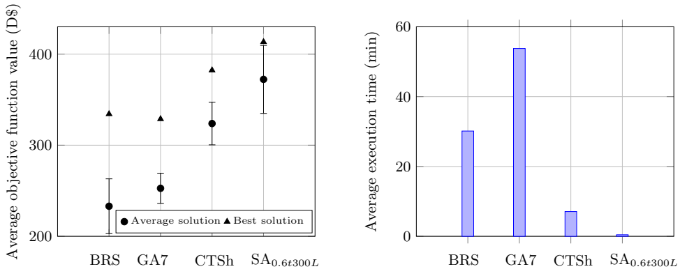
(a) Best and average solutions of the best four metaheuristic approaches. The error bars indicate one standard deviation around the average objective function value.
