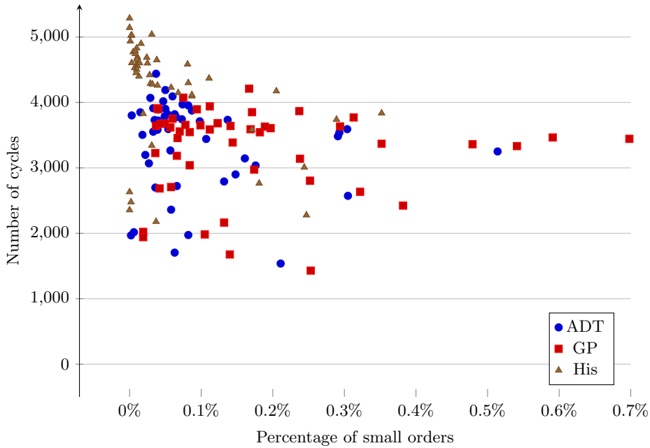
Figure 3: A scatter plot between the number of cycles traversed and the percentage of the total picked volume attributed to small orders. Each marker represents a single problem instance with four picking lines.
