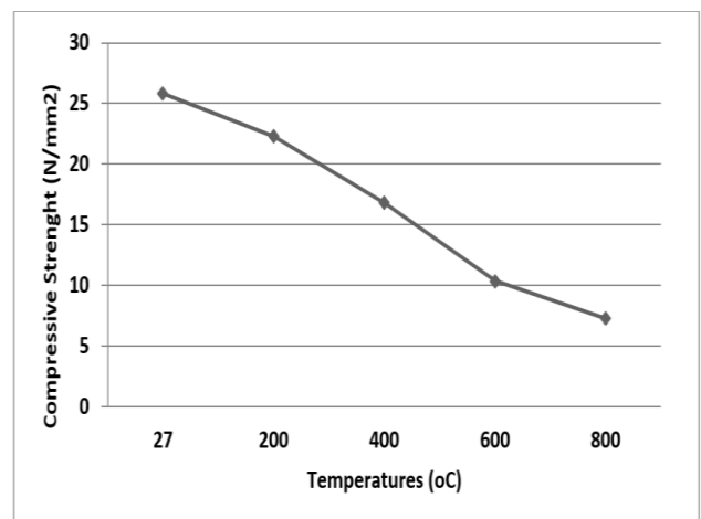
Figure 2: Residual Compressive Strength of Metakaolin Geopolymer Concrete
