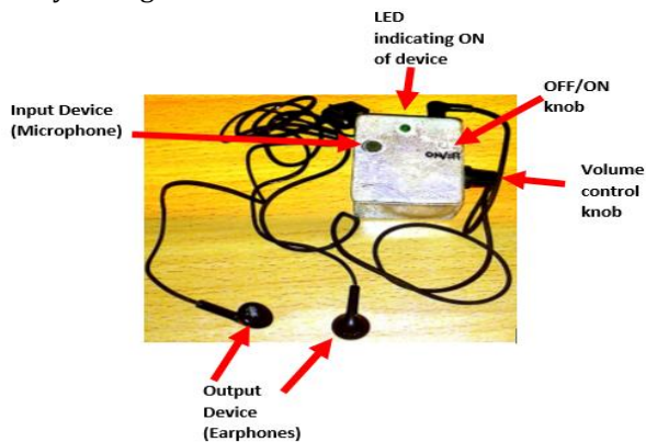
Figure 11: Packaged prototype of the digital hearing aid.
