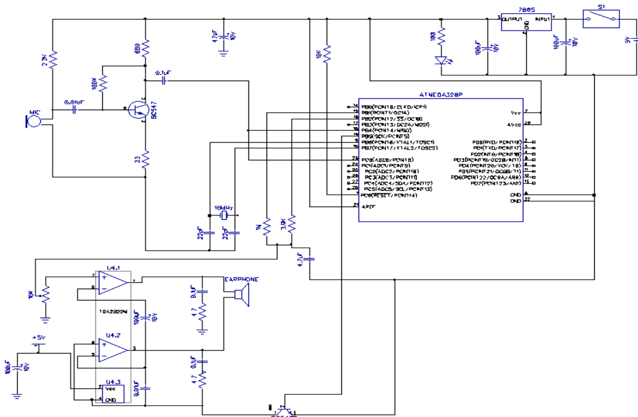
Figure 10: The overall circuit diagram of the hearing aid system
