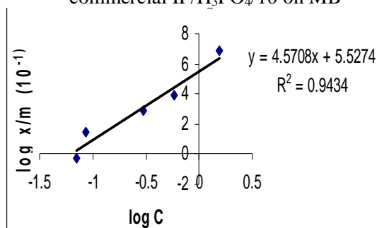
Fig. 6: Freundlich adsorption isotherm of < 2 mm IP/ZnCl 2 /10 on MB
