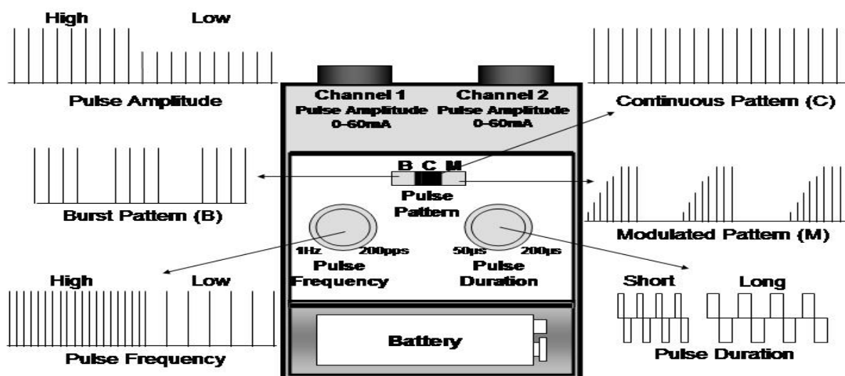
Figure 3: Output characteristics (settings) of a standard TENS device. The user can control the amplitude (intensity), duration (width), frequency (rate) and pattern (mode) of the pulsed electrical currents.
