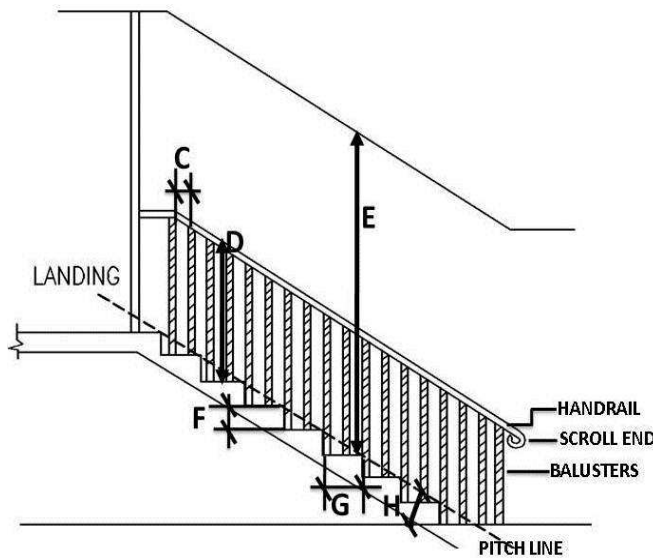
Fig. 3: Typical elevation showing components of stairs
