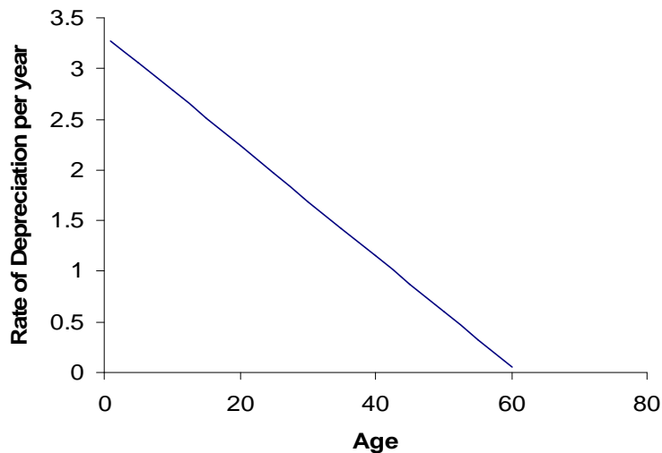
Fig. 1: Sum of the Years' Digits Depreciation path
