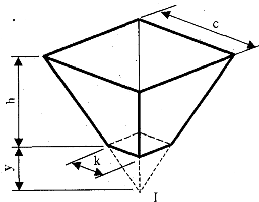
Fig. 1: Hopper Design
