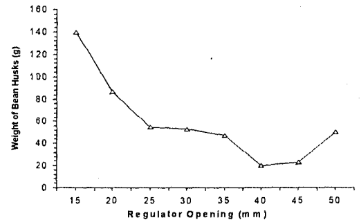
Fig. 6: Variation of Weight of Bean Husks with Regulator Opening
