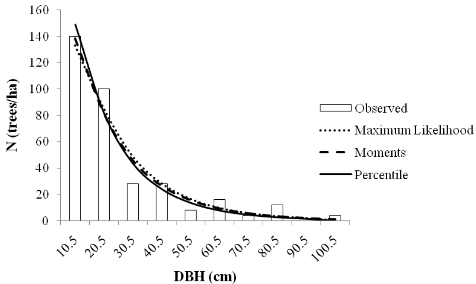
Fig. 3: Observed diameter distributions, fitted 3-parameter Weibull distribution by maximum likelihood, moments and percentile methods in number of trees per ha for two plots.
