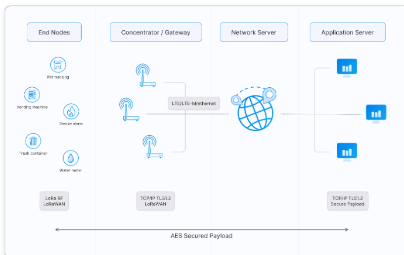
Fig.6. LoRa architecture
