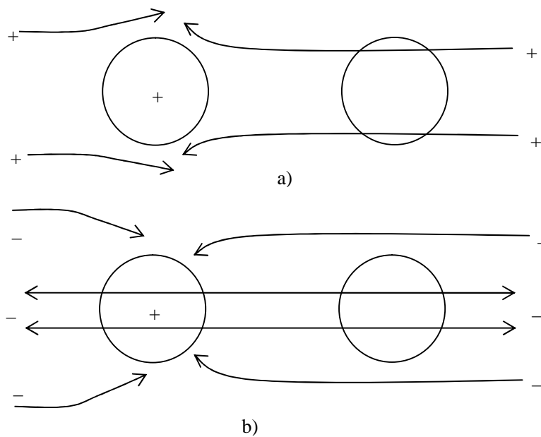
Fig.1. The lines of motion of the small particles of the vacuum field, which are a) positively charged, b) negatively charged, near two bodies one of which is neutral and the other is positively charged
