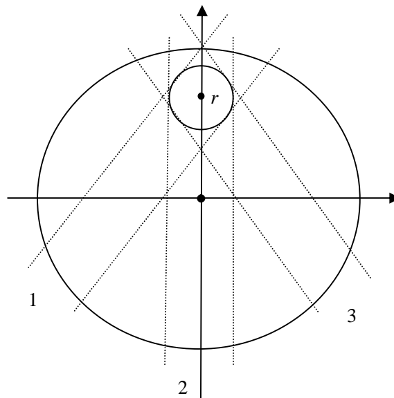
Fig.5. The small ball is at a distance r from the center of the large ball.
