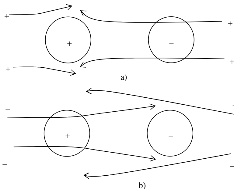
Fig.2. The lines of motion of the small particles of the vacuum field which are a) positively charged, b) negatively charged, near two bodies, one of which is negatively charged and the other is positively charged
