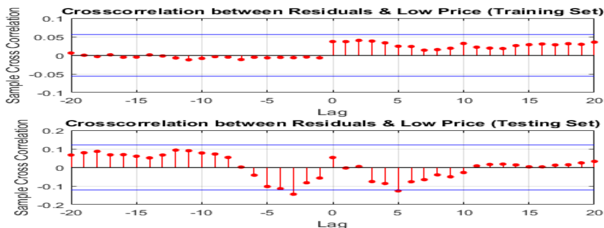
Fig.12. Cross-correlation between residuals and low price for training and testing sets
