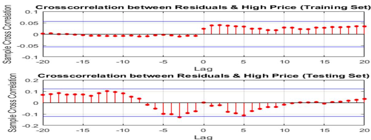
Fig.11. Cross-correlation between residuals and high price for training and testing sets
