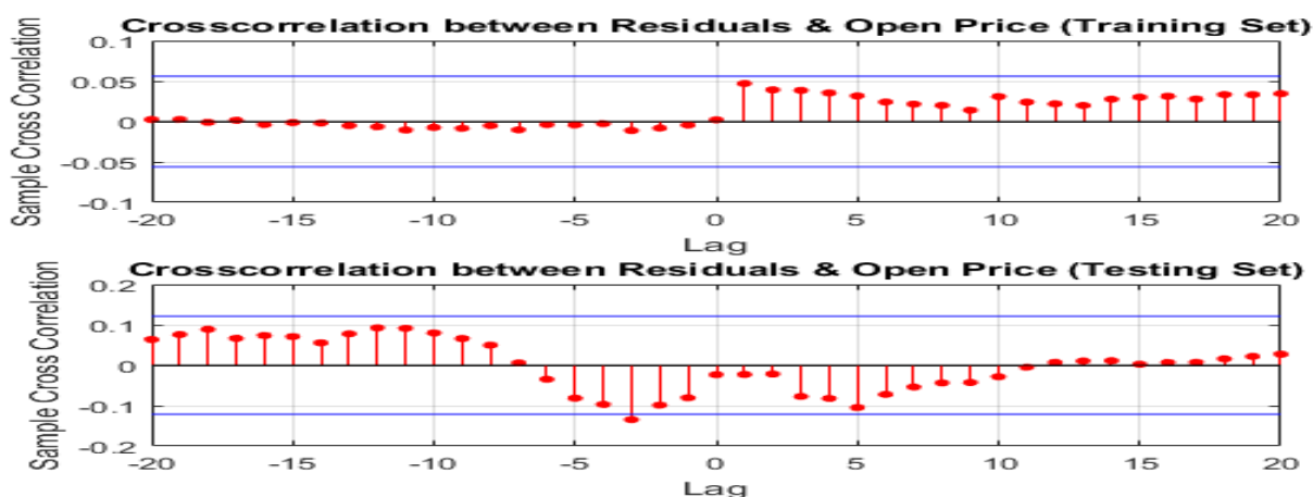
Fig.10. Cross-correlation between residuals and open price for training and testing sets
