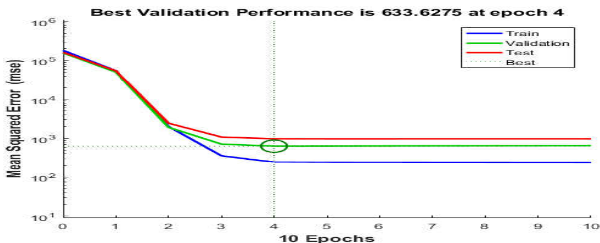
Fig.1.MLP training performance
