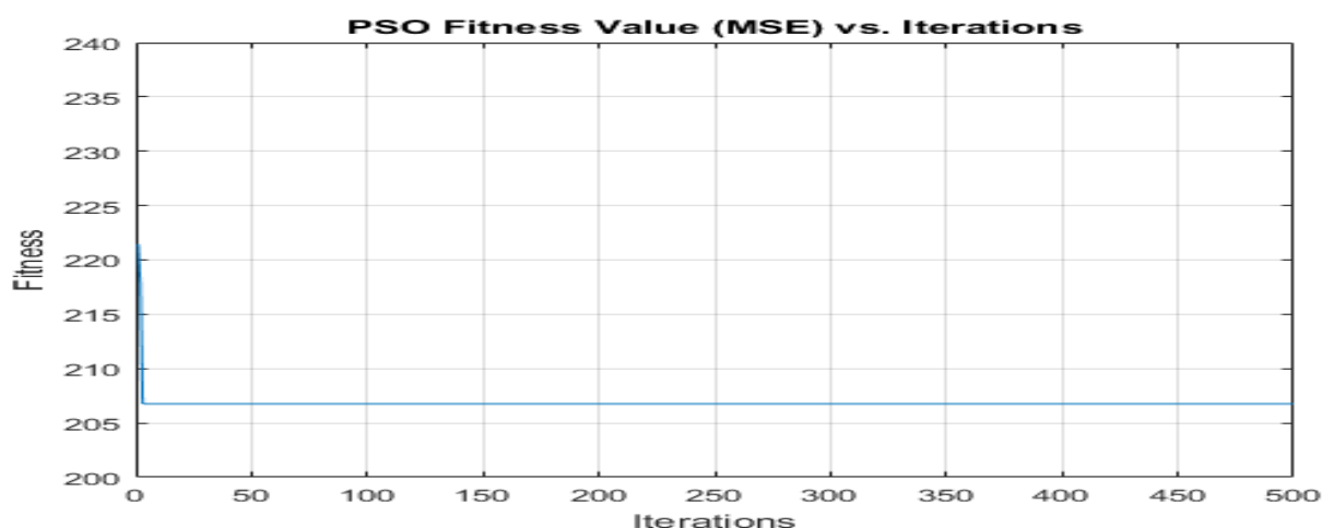
Fig.1.PSO optimization plot
