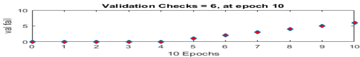
Fig.2. Training stopped after six consecutive increases in validation set error
