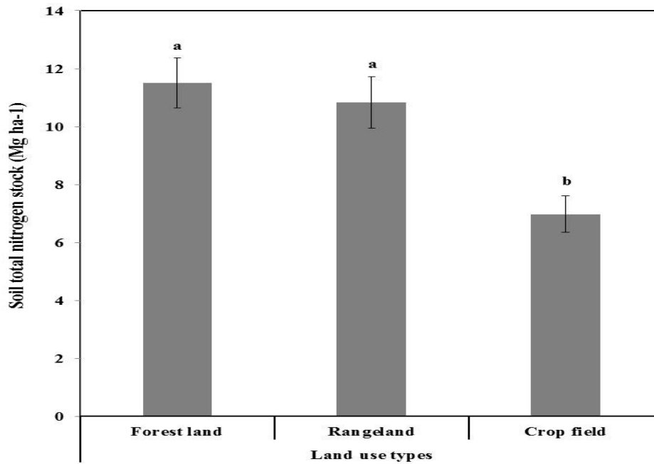
Fig. 3 Soil nitrogen (SN) stock in different land unit under surface erosion. Different letters indicate that SN stock is significantly different at 1% level based on Tukey HSD Post-hoc test.
