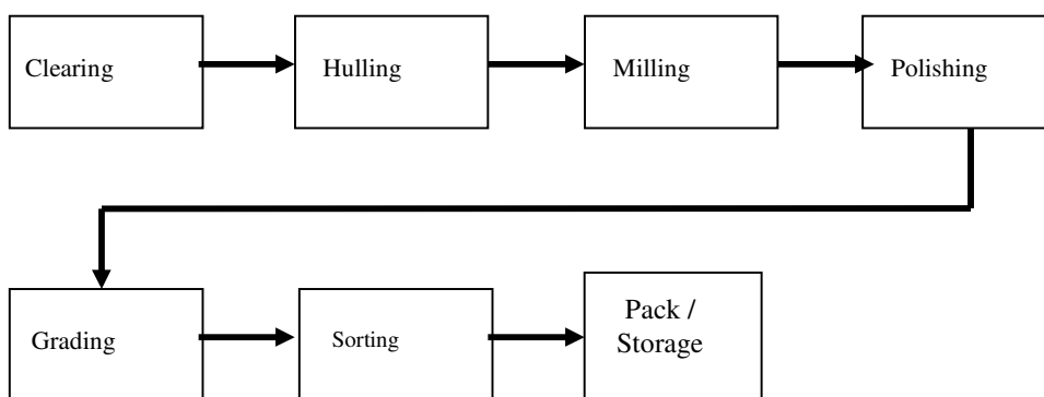
Fig. 1: Summary Chart for Rice Milling Process
