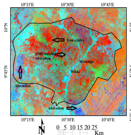
Fig 4: Landsat 8 band ratio 7/5, 5/4, 6/7 image for Yankari scene and environs
