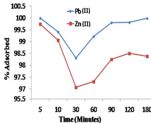
Fig. 2: Effect of contact time on the Pb (II) and Zn (II) ions, biosorption on plantain stalk ( Musa paradisiaca )
