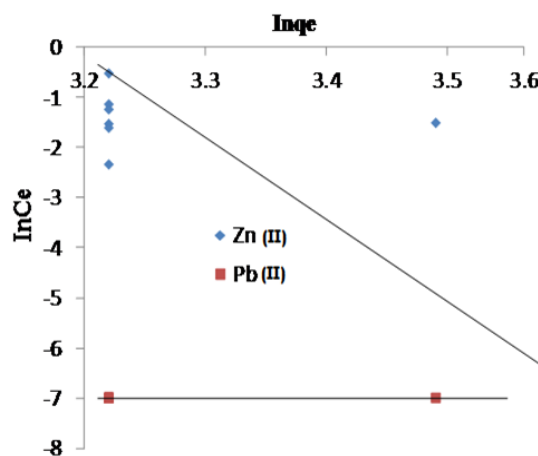
Fig. 7: Freundlich equilibrium isotherm for the sorption of Pb (II) and Zn (II) ions by plantain stalk ( Musa paradisiaca )
