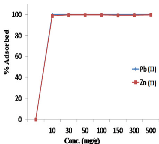
Fig. 3: Effect of concentration on the Pb (II) and Zn (II) ions biosorption on plantain stalk ( Musa paradisiaca )
