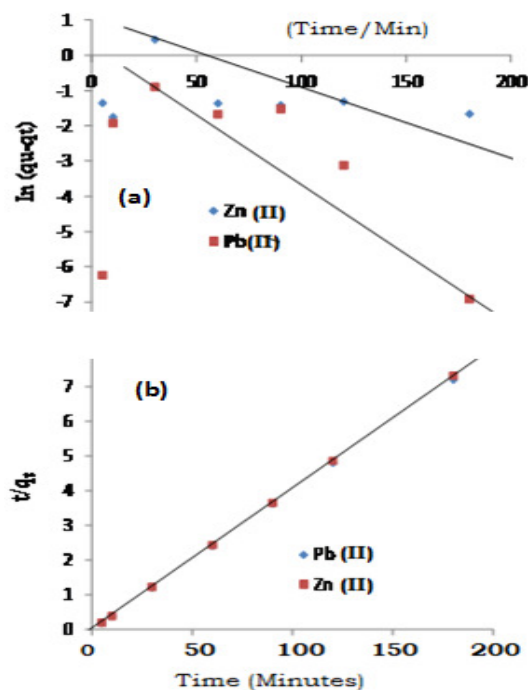
Fig. 8 (a) and (b): Pseudo-first and second-order kinetics for the sorption of Pb (II and Zn (II) ions by ( Musa Paradisiaca )
