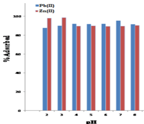
Fig. 1: Effect of pH on Pb (II) and Zn (II) ions biosorption on plantain stalk ( Musa paradisiaca )
