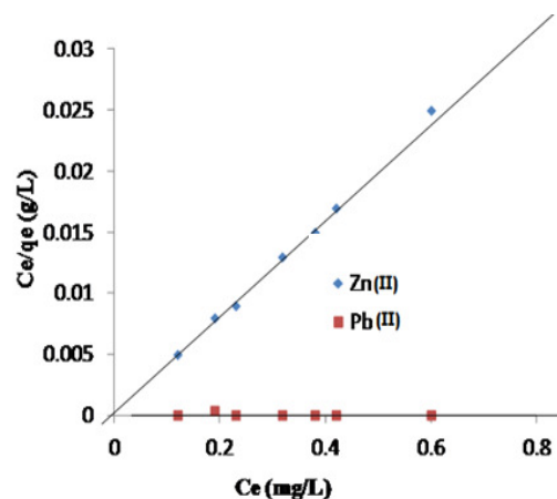
Fig. 6: Linear Langmuir Adsorption isotherm for metal ion removal from aqueous solution by plantain stalk ( Musa paradisiaca )
