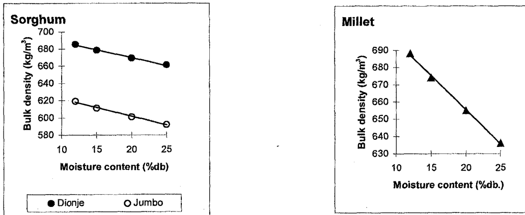
Figure 3: The effect of moisture content on bulk density of sorghum and millet.
