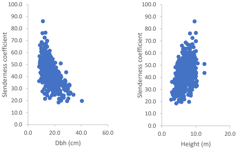
Fig. 2: Relationship of TSC with DBH and Height for Gmelina stand.
