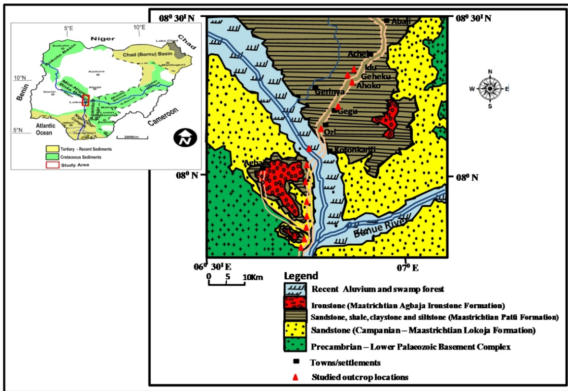
Figure 1: Geological Map of Study Area Showing Locations of Studied Sections with Inset Map of Nigeria Showing NW/SE Trending Bida Basin (Modified After Agyingi, 1991)
