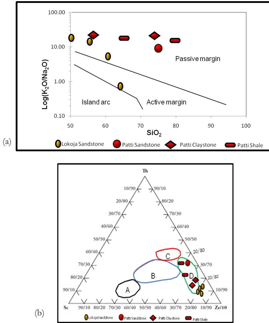
Fig. 12: (a) Plot of the \log(K_2O/Na_2O) against SiO_2 Discrimination Diagram for Sandstone-Mudstone Suites Showing the Fields for a Passive Continental Margin, an Active Continental Margin and an Island Arc (After Roser and Korsch, 1986). (b) Th-Sc-Zr/10 Discrimination Diagram (After from Bhatia and Crook, 1986). The fields are: A - Oceanic Island-Arc, B - Continental Island-Arc, C - Active Continental Margin, D - Passive Margin
