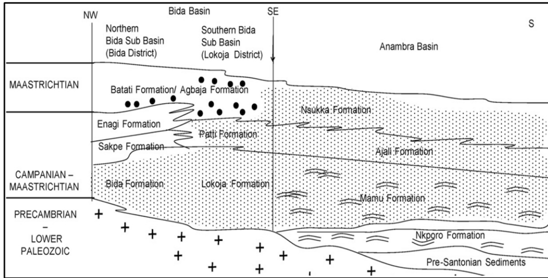
Fig. 2: Regional Stratigraphic Successions in the Bida Basin and Restored NW-SE-S Stratigraphic Relationships from the Bida Basin to the Anambra Basin (After Akande et al. , 2005)
