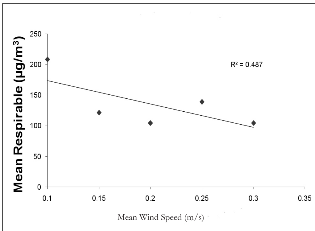
Fig. 2: Correlation of Mean Respirable Particle with Mean Wind Speed (Scatter Plot)
