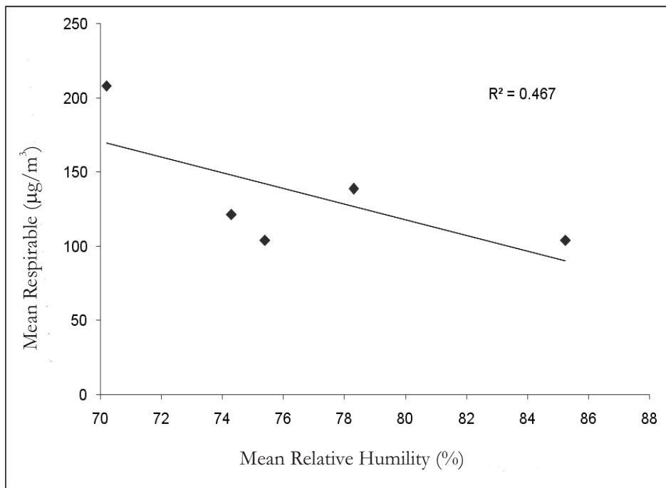
Fig.4: Correlation of Mean Respirable Particle with Mean Relative Humidity (Scatter Plot)
