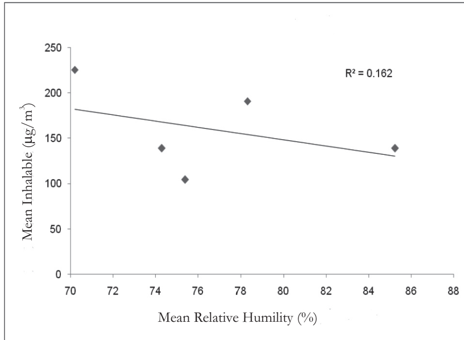
Fig. 5: Correlation of Mean Inhalable Particle with Mean Relative Humidity (Scatter Plot)
