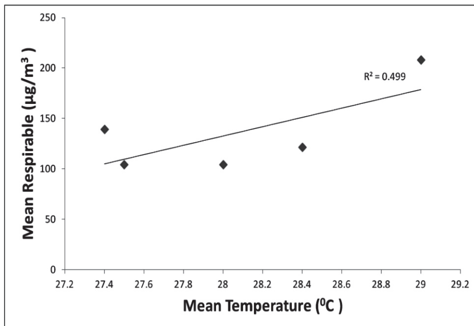
Fig 6: Correlation of Mean Respirable with Mean Temperature (Scatter Plot)
