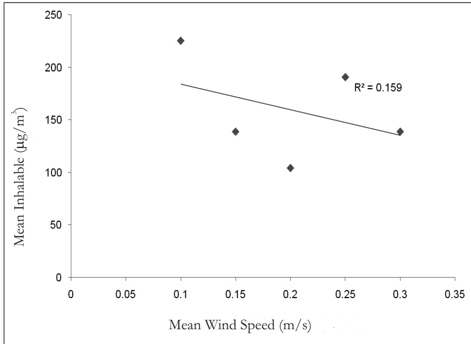
Fig. 3: Correlation of Mean Inhalable Particle with Mean Wind Speed (Scatter Plot)
