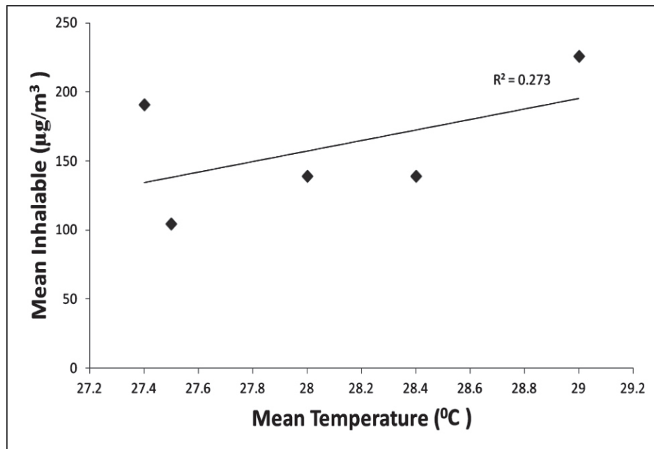
Fig 7: Correlation of Mean Inhalable with Mean Temperature (Scatter Plot)
