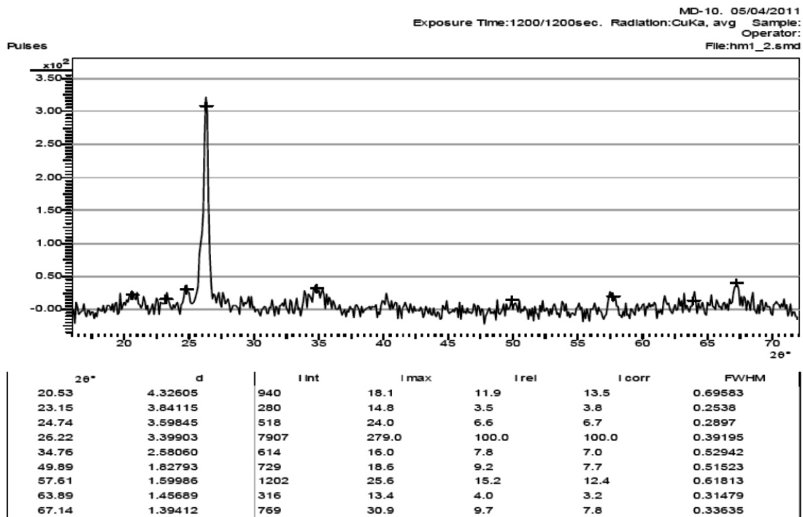
Figure 2: Typical X-ray Diffraction Result of the Harmattan Dust Sample Collected Showing a Single Peak.
