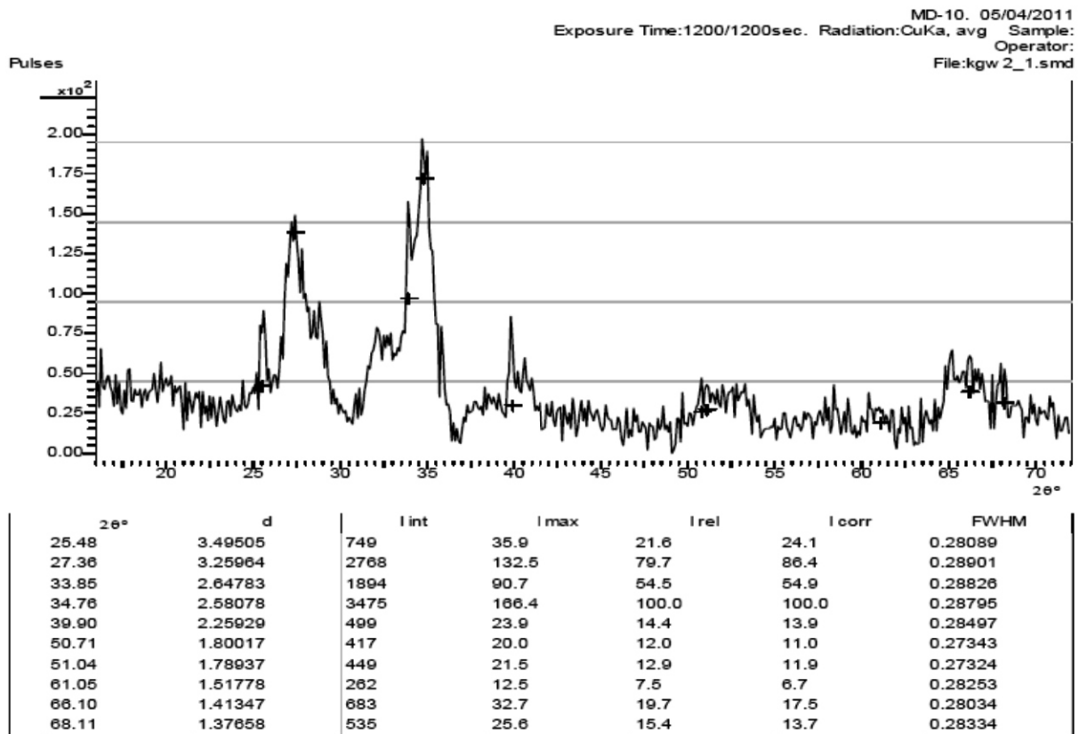
Figure 3: Typical X-ray Diffraction Result of the Harmattan Dust Sample Collected Showing Multiple Peaks.
