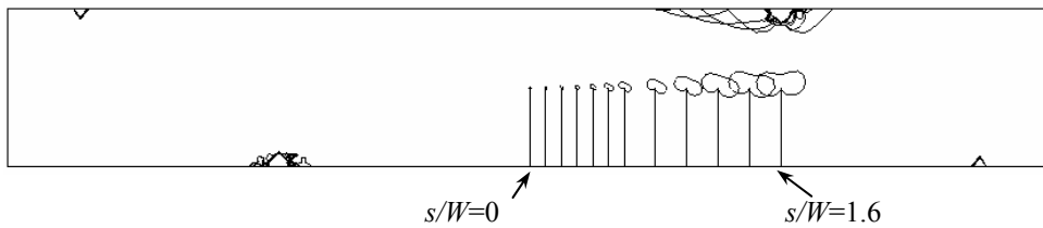
Figure 8. Typical plastic zone contours for s/W=0-1.6 and a/W=0.5 for applied load 2 kN.
