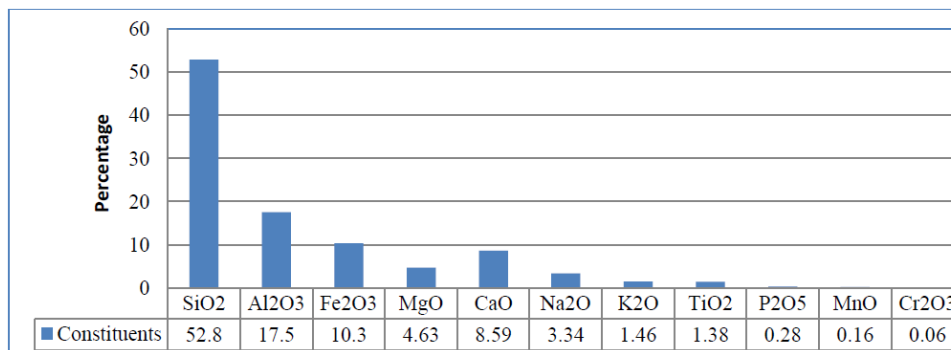
Fig. 4. Chemical composition of basalt fiber
