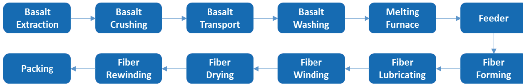
Fig.2 Flow chart of basalt fiber production
