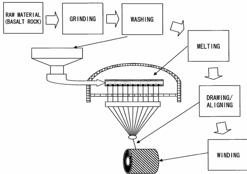
Fig.-1 Plant layout of Basalt Fiber Production
