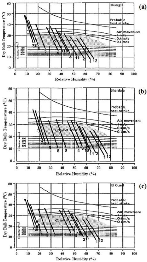
Figure 5. Olgyay Bioclimatic chart of (a) Ouargla, (b) Ghardaia, and (c) El Oued
