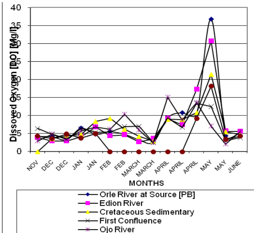
Figure 1: Seasonal Variation in Dissolved Oxygen (DO) [Mg/l] in Orle River Basin
