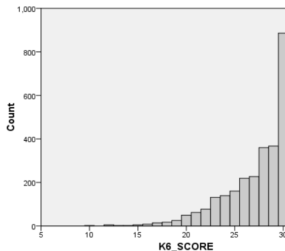
Figure 1 K6 Distribution
