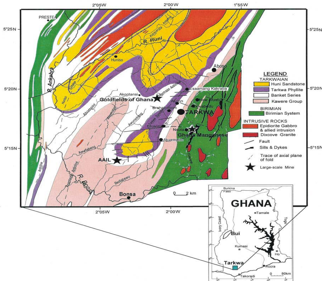
Fig.2 Simplified Geological Map of the Tarkwa Area (Modified from Junner et al , 1942)
