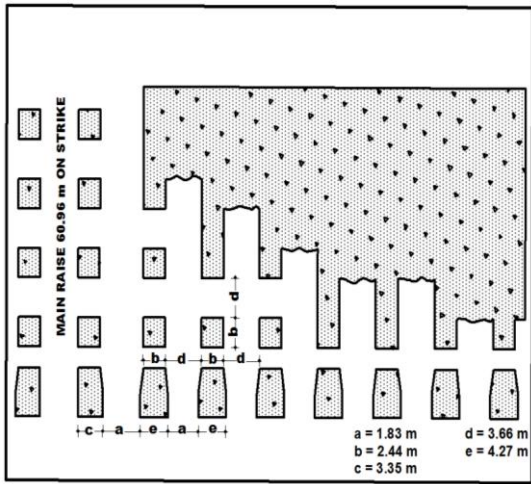
Fig. 3 Standard Layout for Pillars at GGL (modified from Acquah, 1997).
