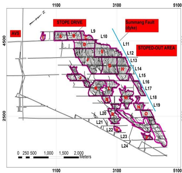
Fig. 4 Longitudinal Vertical Projection of Stopped-out Areas in the WL-WR Compartment of the AVS.
