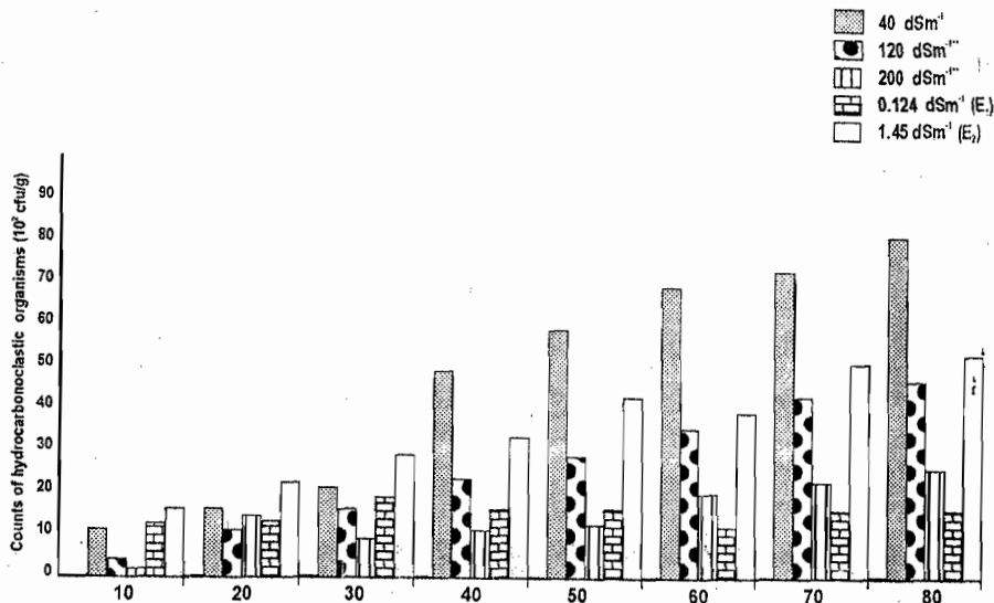
Fig. 1: Influence of electrical conductivity (EC) on numbers of hydrocarbonoclastic microorganisms in Crude oil contaminated soil.
