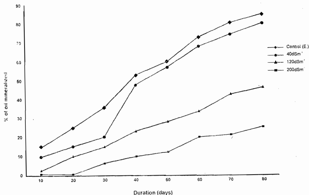
Fig. 2 Influence of electrical conductivity on mineralization of crude oil in ultisol
