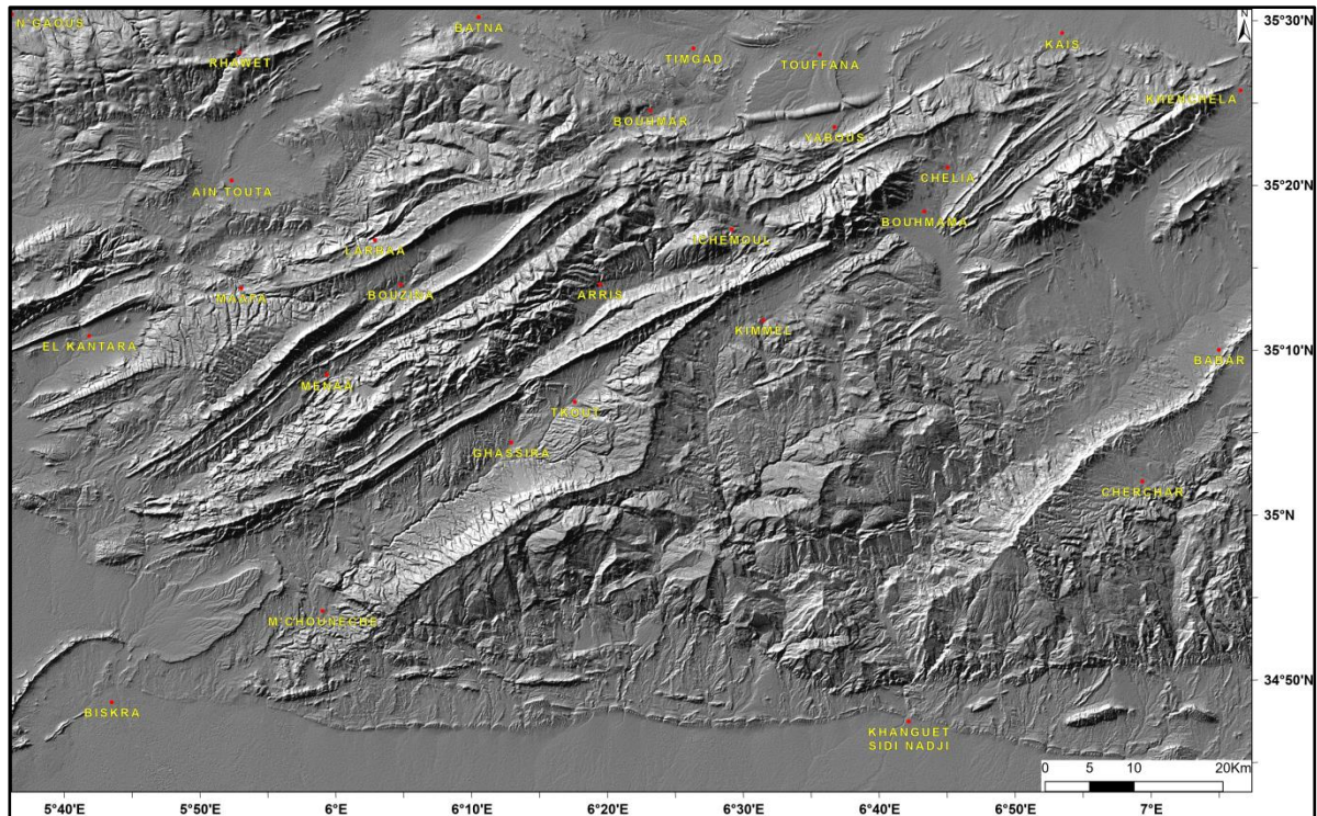
Fig. 5 Grey shaded relief derived from SRTM data with 135° solar azimuth
