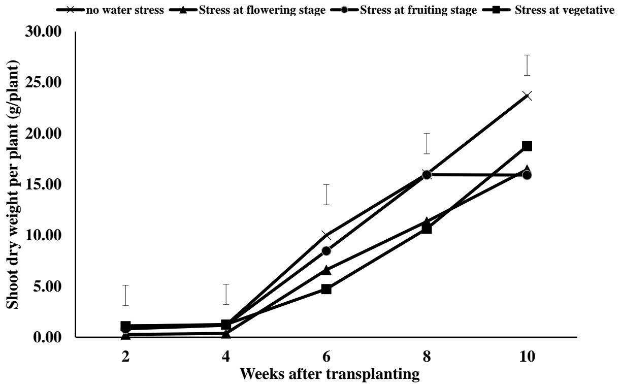
Figure 4: Shoot dry weight of tomato as influenced by water stress at different phenological stages (Error bars denote LSD)
