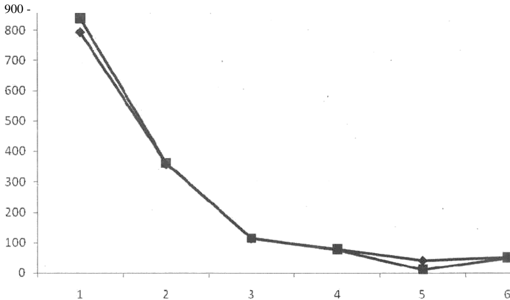
Figure 2: Observed and Predicted species distribution for 1962 using X^2 - test statistics
