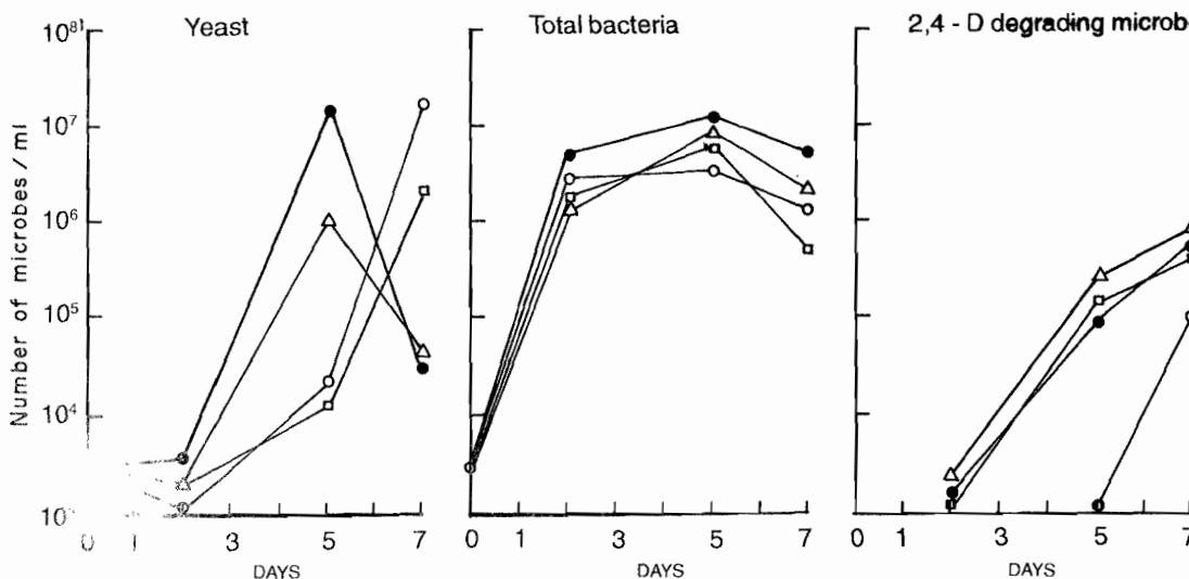
Fig. 4. Changes in microbial population in perfusate of soils amended with N (●), P (▲) and K (□), and control (○).
