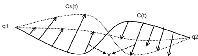
Fig.1. Variations C_s and infinitesimal variations X of a curve C with end points q_1 and q_2
