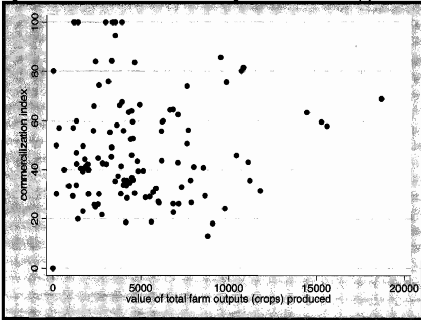
Figure 4: Plot of commercialisation index against total value of crop production
