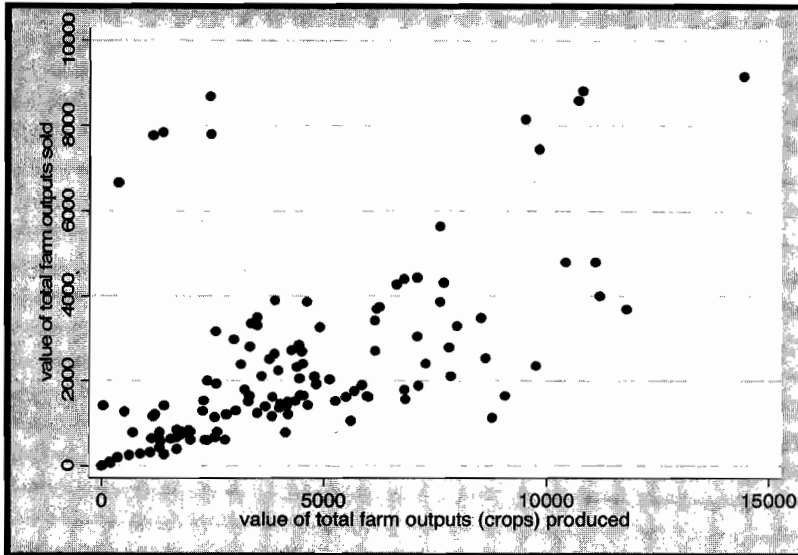
Figure 3: Scatter plot of value sold against value produced 14
