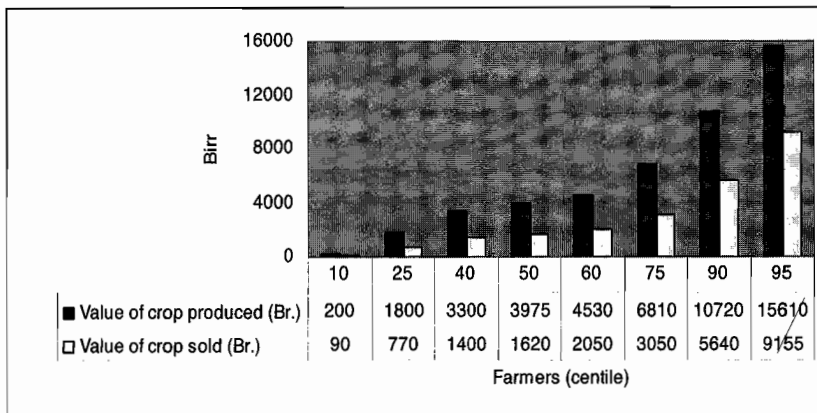
Figure 2: The relationship between crop value produced and sold
