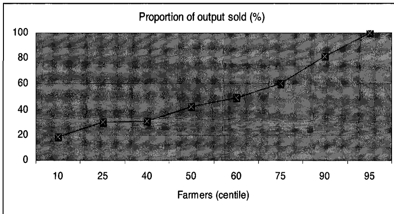
Figure 1: Proportion of output sold
