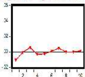
Response of NET_GOVERNMENT_REVENUE to CAPITAL_EXPENDITURE
