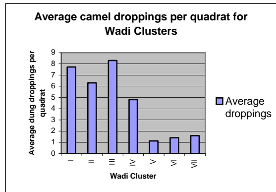
Figure 11: Average number of dung droppings per quadrat for (a) camel, (b) goat, (c) donkey, (d) ibex, (e) fox, grouped by TWINSPAN wadi clusters.
