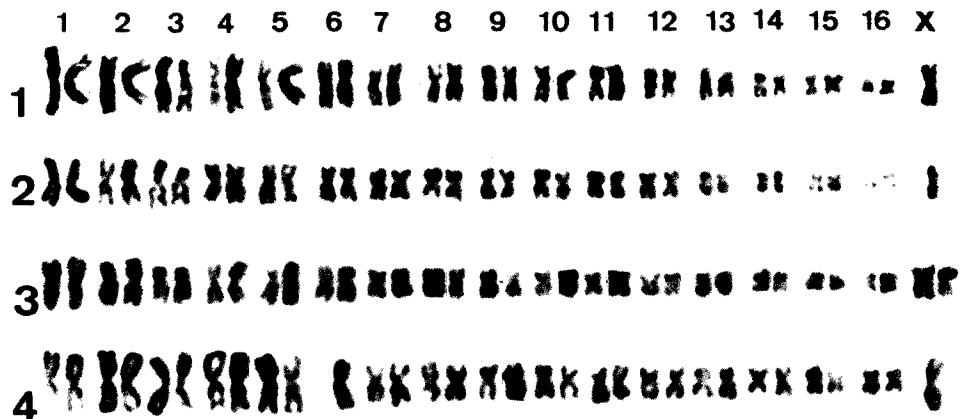
Figure 1: Mitotic chromosomes of Hydrovatus cuspidatus . 1, 2, 3, 4 males, mid-gut nuclei, unbanded. The autosomes 1 to 6 are mostly metacentric while 7 to 16 are slightly submetacentric and show apparently gradual decrease in size. The X chromosome is clearly metacentric. 1, 2, 3 Corsican material, 4, Egyptian material. Karyotype with simple sex chromosome system 2n = 2n = 33 (16 + X0) in males and in 2n = 34 (16 + XX) in females. Scale line represents 5\mu\text{m} .
