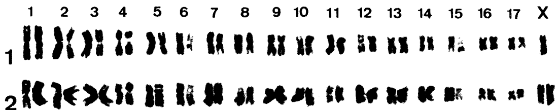
Figure 2: Mitotic chromosomes of Hydroporus humilis . 1, male, mid-gut nuclei, unbanded. 2, female, ovary, unbanded. The autosomes are mainly metacentric or nearly so. The first two pairs of autosomes are almost equal in length and the largest element in the nucleus. The rest of the autosomes show fairly gradual decrease in size. X chromosome is submetacentric and clearly larger than the last autosomal pair. Karyotype with simple sex chromosome system 2n = 35 (17 + X0) in males and 2n = 36 (17 + XX) in females. Scale line represents 5\mu\text{m} .
