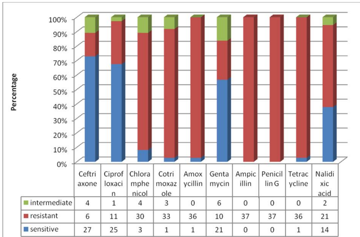
Figure 2: Sensitivity patterns of Klebsiella spp obtained from peritoneal fluid cultures (n=37****) ****Includes the 4 cases of Klebsiella spp among those with more than one peritoneal fluid isolate
