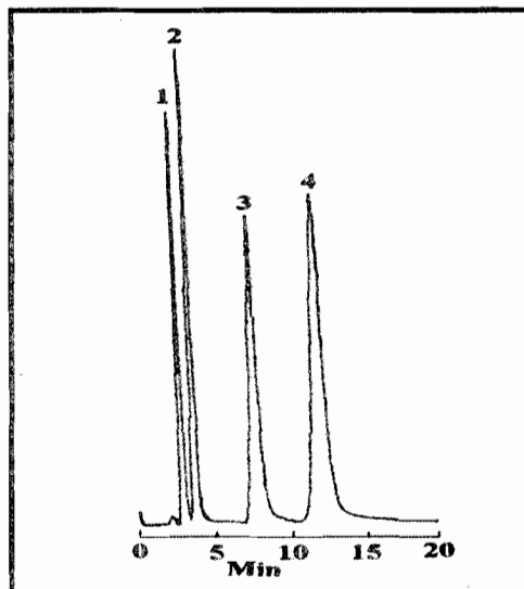
Figure 5. A typical chromatogram of phenobarbitone (1) 0.6 \mu g, ethosuximide (2) 5.0 \mu g, phenytoin (3) 0.6 \mu g and carbamazepine (4) 0.3 \mu g on PLRP-S 100Å 8 \mu m column. Column temperature: 60 °C Mobile phase: Acetonitrile- tert -butanol-phosphate buffer (pH 7.6, 0.2 M) - water (25:5:10:60, v/v) Flow rate: 1 ml/min. Detection: UV at 220 nm.
