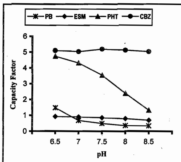
Figure 3. Effect of mobile phase pH on capacity factors of phenobarbitone (PB), etho-suximide (ESM), phenytoin (PHT) and carbamazepine (CBZ). Mobile phase: Acetonitrile- tert -butanol-phosphate buffer (pH 7.5, 0.2 M) - water (25:X: 10: 65-X, v/v). Flow rate: 1 ml/min. Column: PLRP-S 8 \mu m 100 \text{\AA} . Column temperature: 60 ^{\circ} C. Detection: UV at 220 nm.
