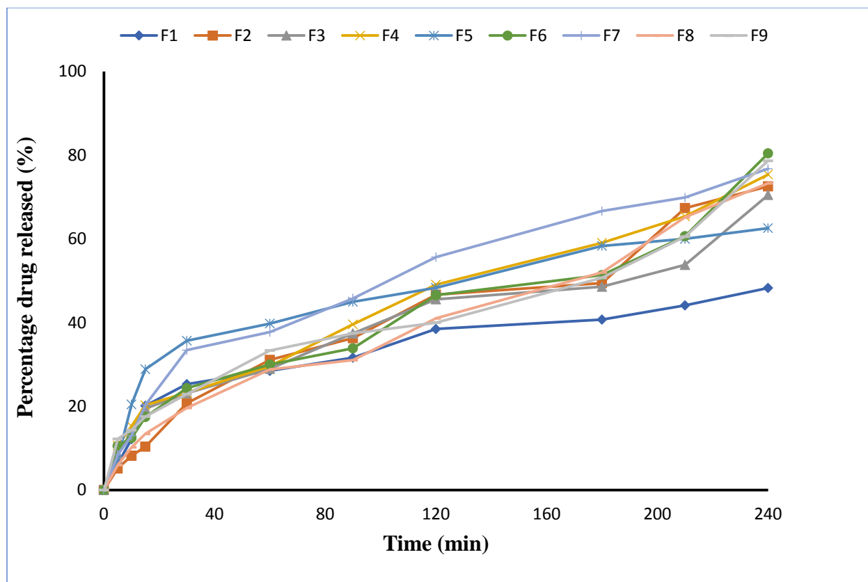
Figure 5: Dissolution profile of metoprolol-loaded microballoon formulation
