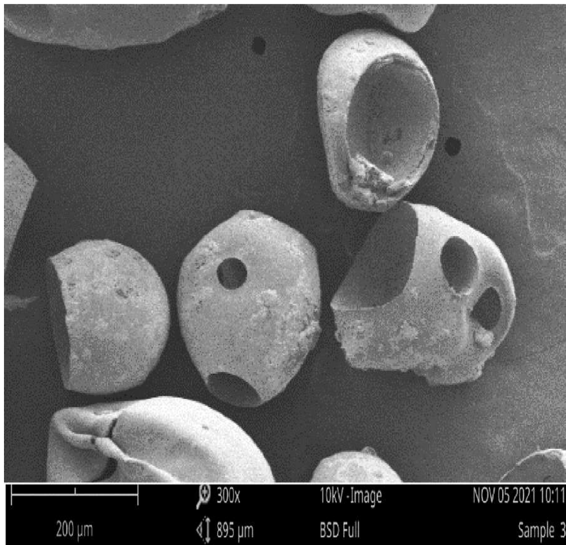
Figure 3. SEM images of microballoons ( \times 300 magnification)
