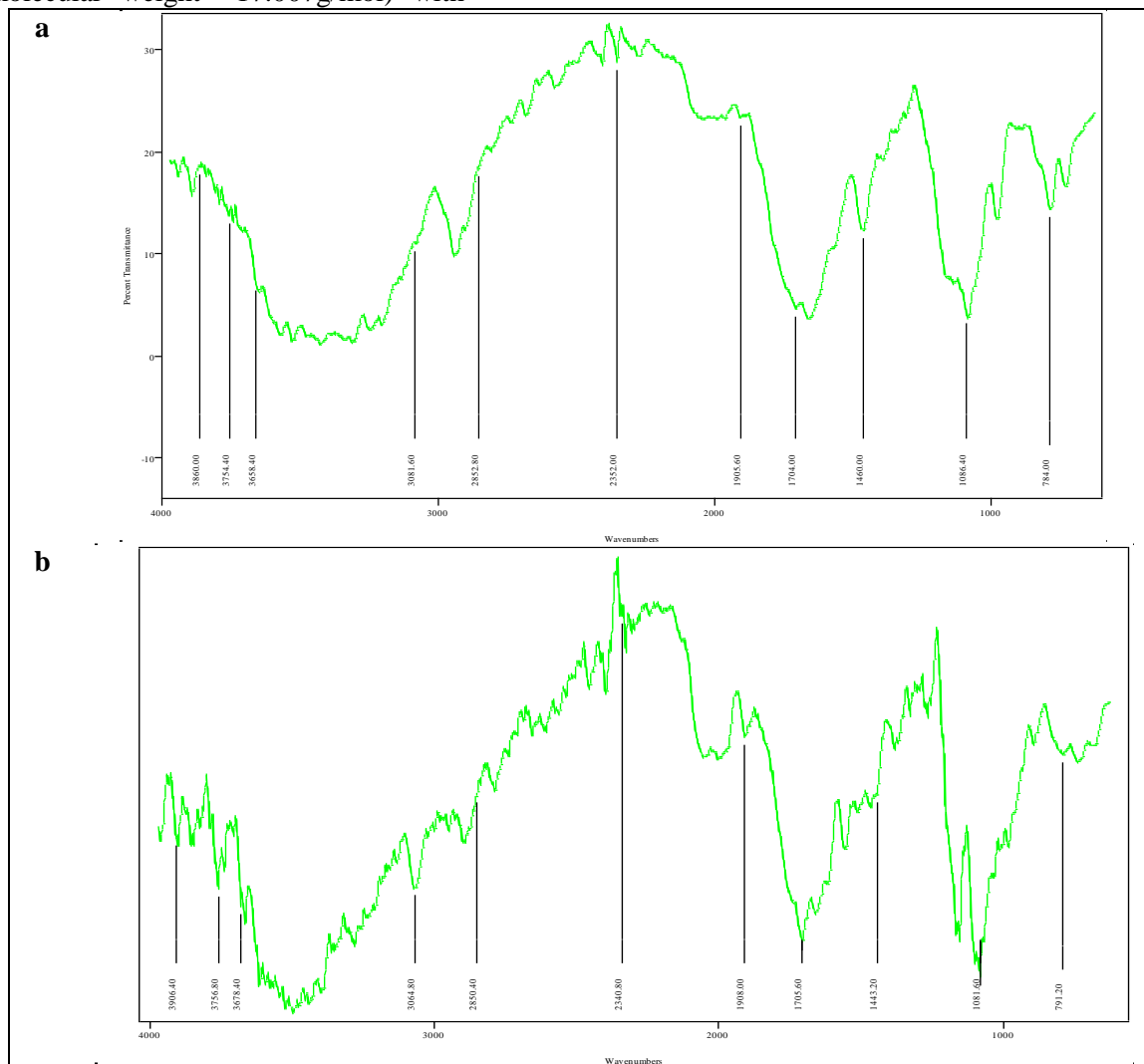
Figure 2: FTIR spectra of (a), native and (b), acetylated cocoyam starches
