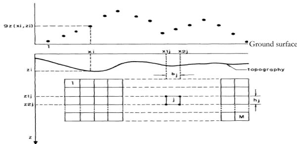
FIG. 1. Gravity field at N points (above) and physical domain discretized into M two-dimensional prisms (below).
