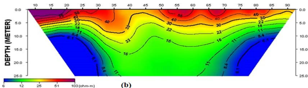
Fig. 14: Fringes and topmost of very low resistivity zones probably composed of laterite with topsoil at traverse 9. Low resistivity ( < 10 \Omega\text{m} ) at a depth of about 9 m downward delineated as peat at the extremes and a trough of clay (resistivity < 30 \Omega\text{m} ) at the middle of traverse 10.
