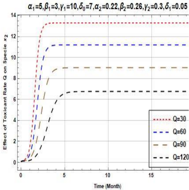
Fig. 2 Effect of Toxicant Flux on Specie Two Concentration
