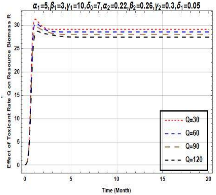
Fig. 3 Effect of Toxicant Flux on Resource Biomass Concentration
