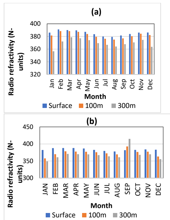
Fig 2: Average seasonal variation of radio refraction at the surface, 100 m and 300 m for (a) 00:00 hour and (b) 12:00 hour.
