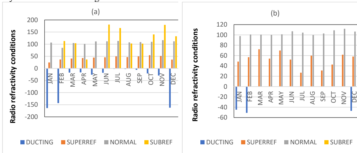
Fig 5: Refractivity conditions in Lagos at (a) 12:00 hour at 0 -100 m and at (b) 12:00 hour at 0-300 m
