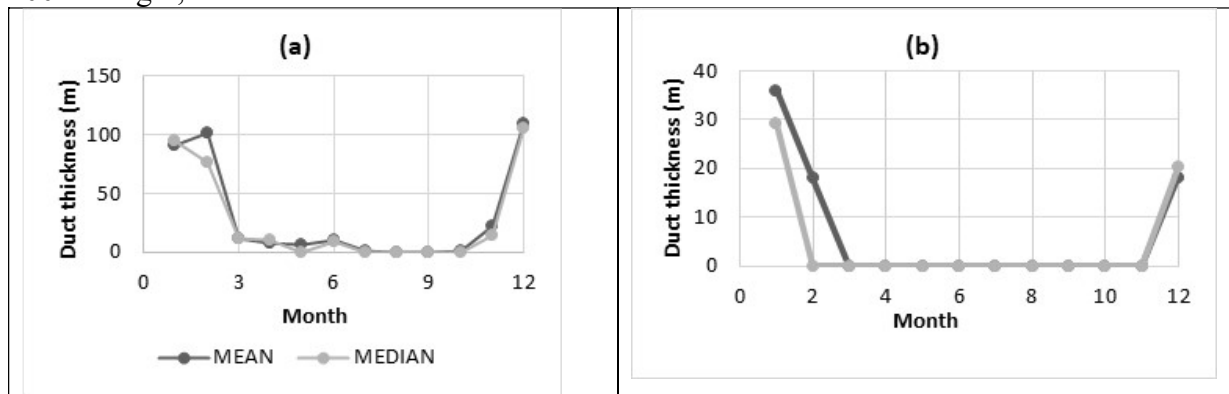
Fig. 10: Monthly variation of duct thickness at 12:00 hour LT over (a) 100 m heights and (b) 300 m heights
