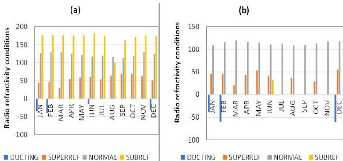
Fig 4: Refractivity conditions in Lagos at (a) 00:00 hour for 0-100m and (b) 00:00 hour for 0-300 m
