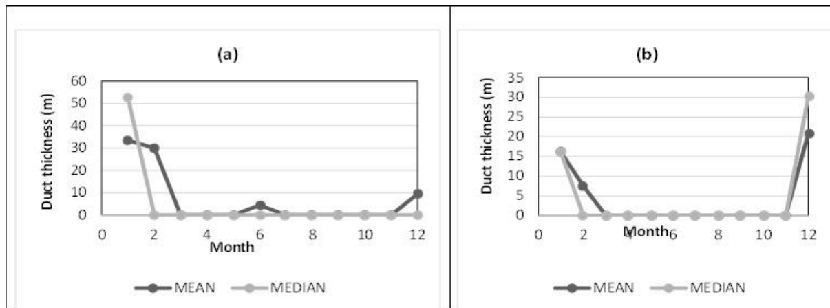
Fig. 8: Monthly variation of duct thickness at 00:00 hour over (a) 100 m heights and (b) 300 m heights
