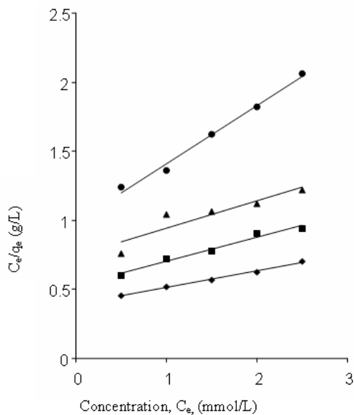
Figure 1. Equilibrium sorption of \text{Zn}^{2+} on activated ( \bullet ) and non-activated ( \blacktriangle ) and \text{Ni}^{2+} on activated ( \blacksquare ) and non-activated ( \blacklozenge ) sugar cane fibre carbon.
