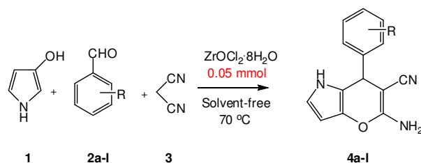
Scheme 1. Synthesis of various 5-amino-7-aryl-6-cyano-4 H -pyrano[3,2- b ]pyrroles.
