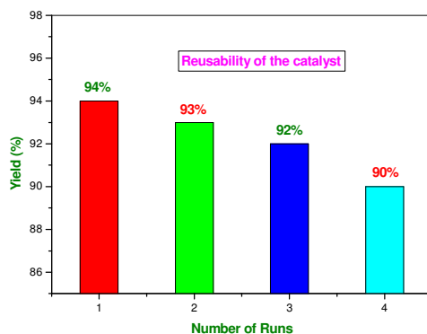
Figure 1. The reusability of the catalyst \text{ZrOCl}_2 \cdot 8\text{H}_2\text{O} for the synthesis of 5-amino-7-aryl-6-cyano-4 H -pyrano[3,2- b ]pyrrole.
